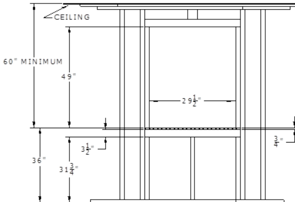
Figure 3-12 ELEVATED FRAMING DIMENSIONS
