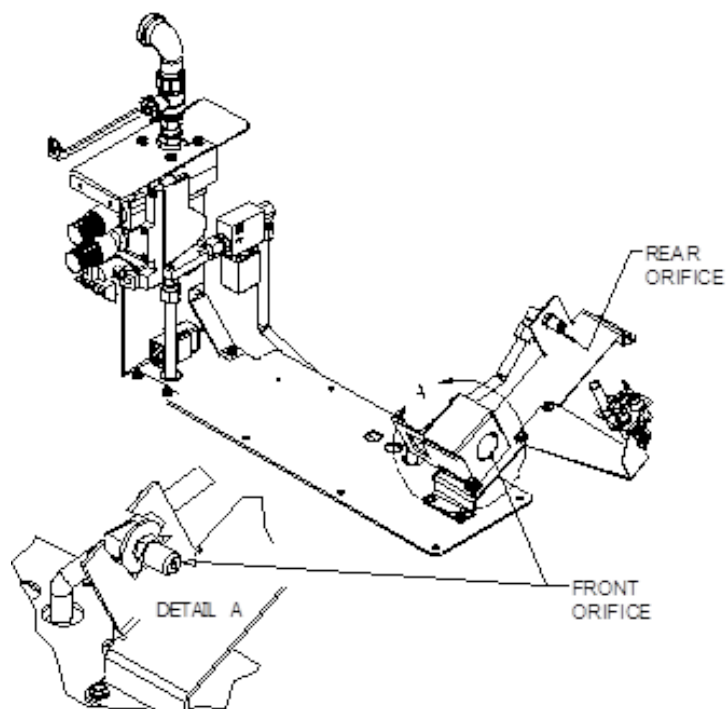
Figure 4-6 Removing Orifices
