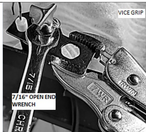
Figure 4-8 Pinch Pilot Base with Vice Grips
