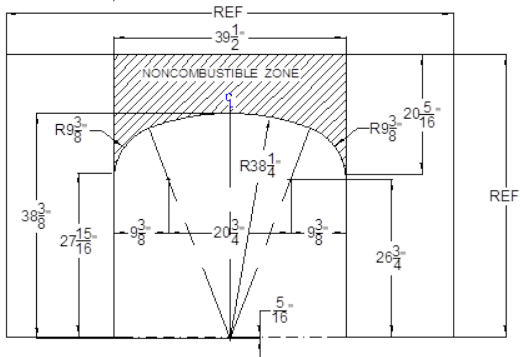
Figure 3-19 NON-COMBUSTIBLE ZONE
